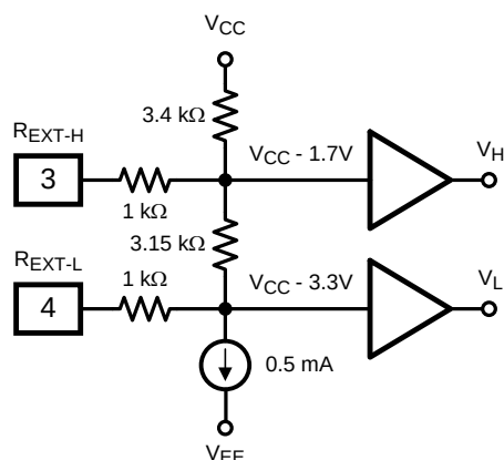
Figure 10. Equivalent Bias Generation Circuit
